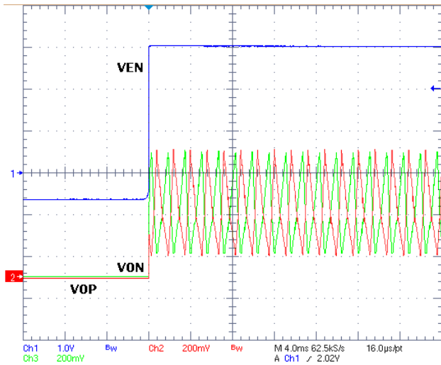
Turn-On time
